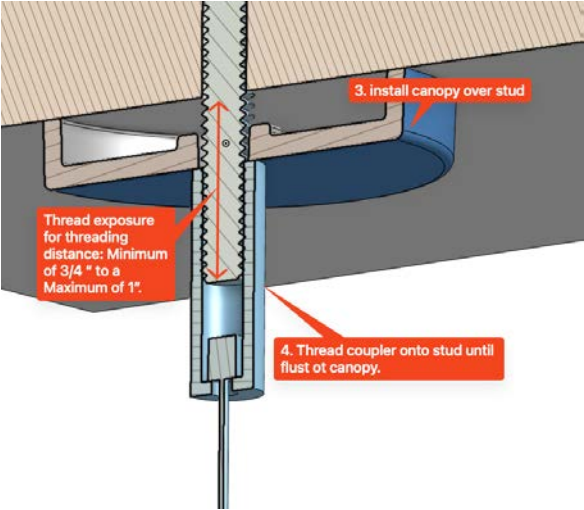
R2 - Recessed Surface Non-Power Mount Kit - Sloped Ceiling
